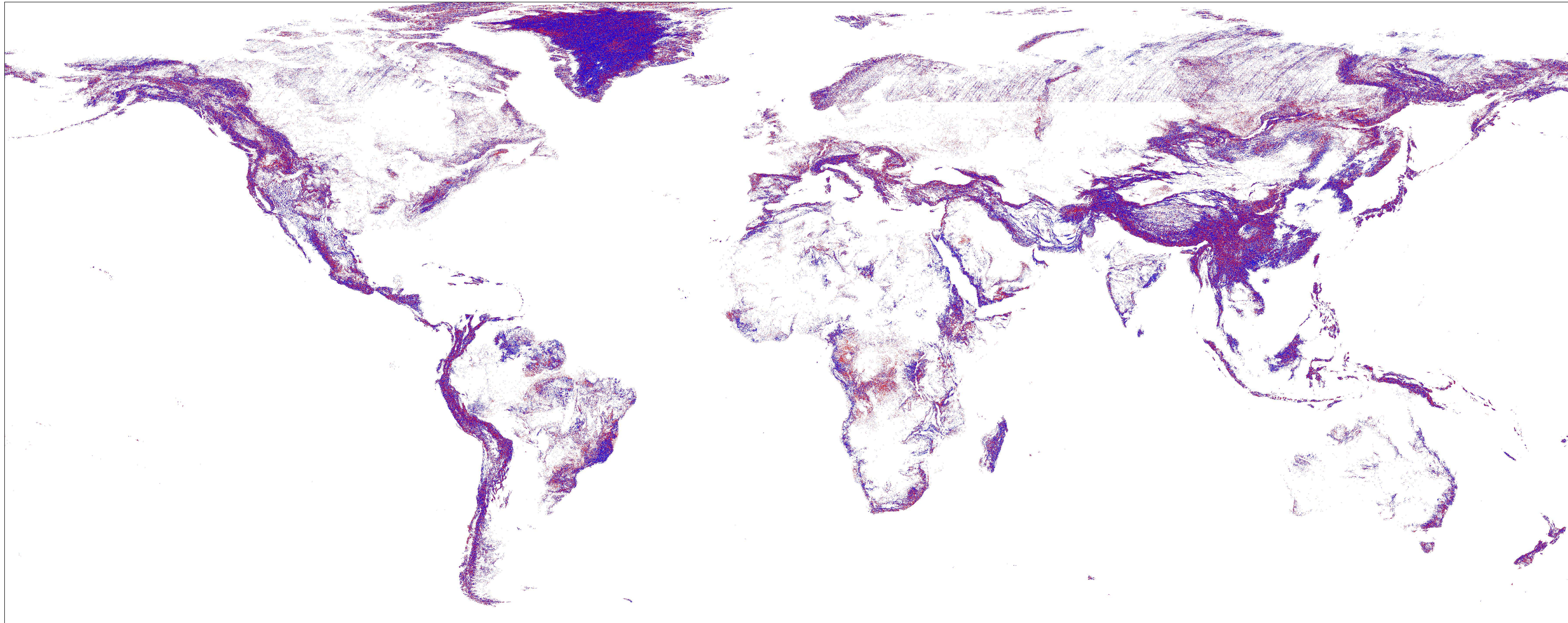
Median topographic position index
