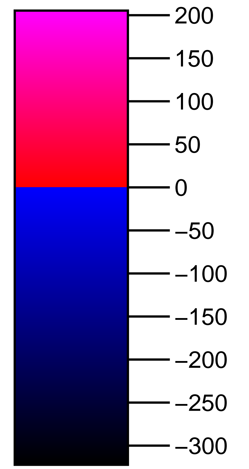
Median topographic position index
