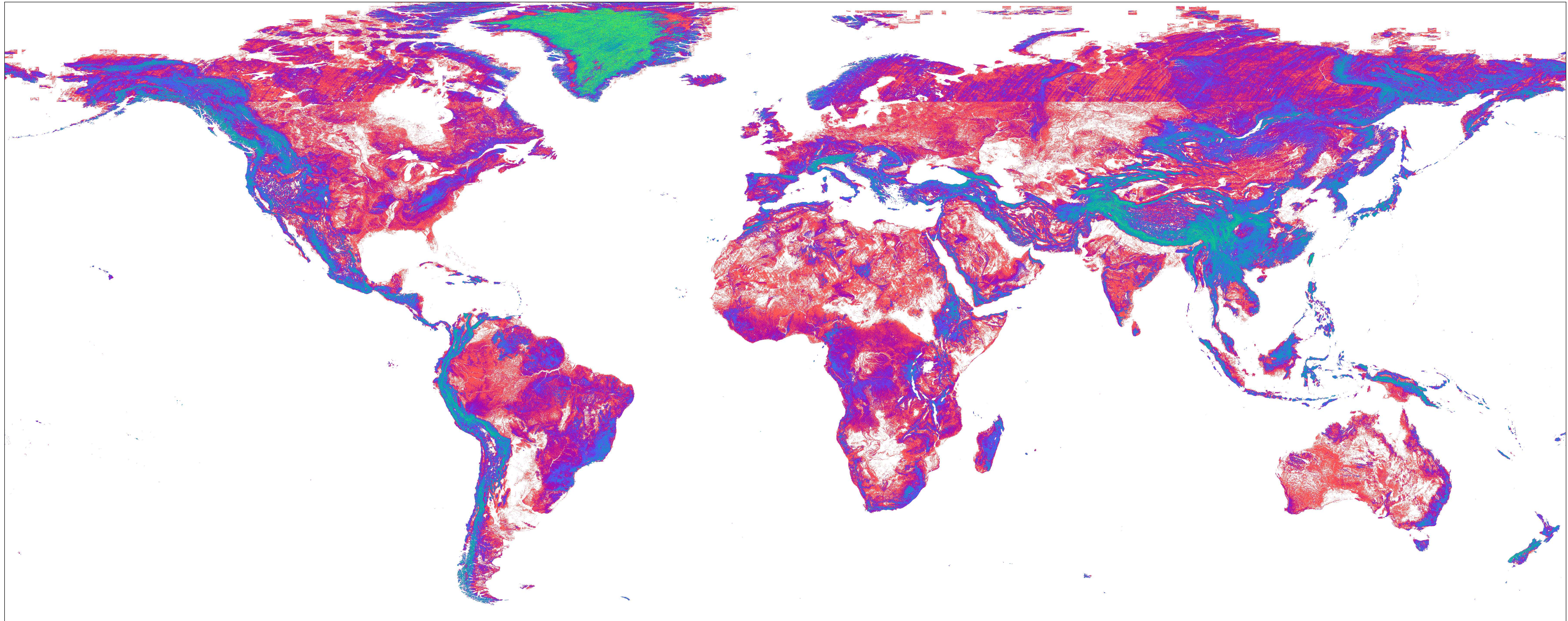
Median terrain ruggedness index
