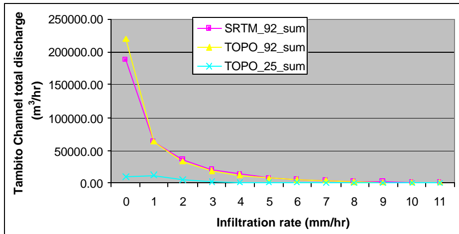
Figure 22. The effect of infiltration rate on runoff for the Tambito main channel for the three digital elevation models.
